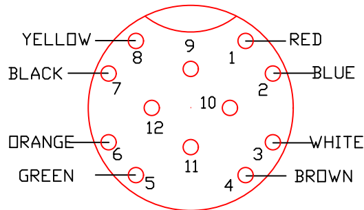
FRONT VIEW OF MATING CONNECTOR. STATOR CABLE WIRE COLORS.
